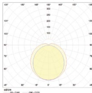
LED T8-840-25W/150cm
