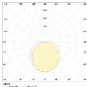
LED T8-840-22W/120cm
