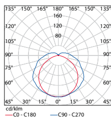
MIRA 2x36W
