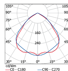
MH3 RX7S
