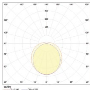
LED T8-840-10W/60cm
